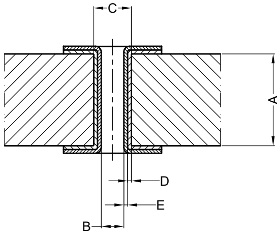
7 PLATED THROUGH-HOLE CROSS SECTION (SCALE 10:1)
